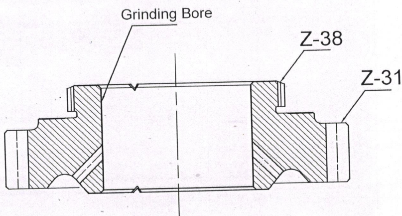
Component Sketch
